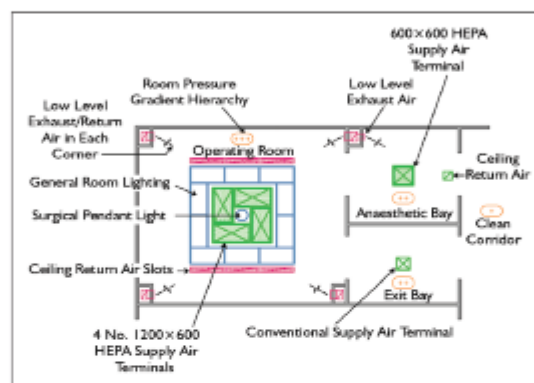
Figure 2: Operating room—plan view of air-distribution system.
